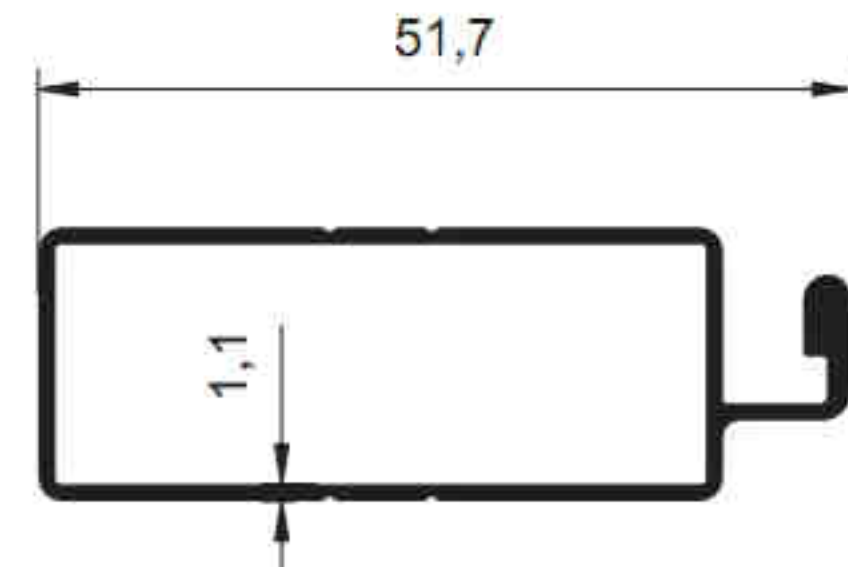
4663 - 0.419 kg/m
