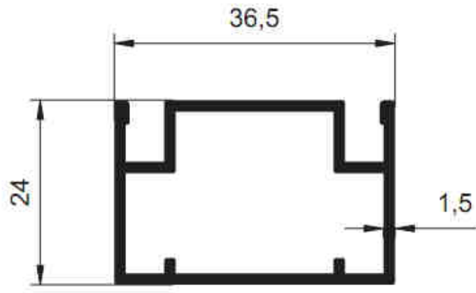
3746 - 0.554 kg/m
