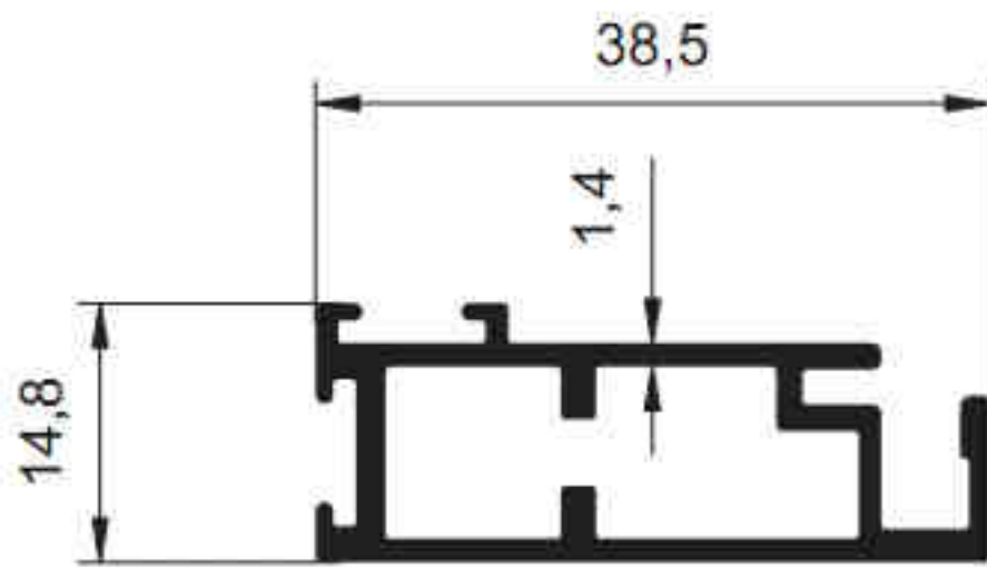
3764 - 0.469 kg/m
